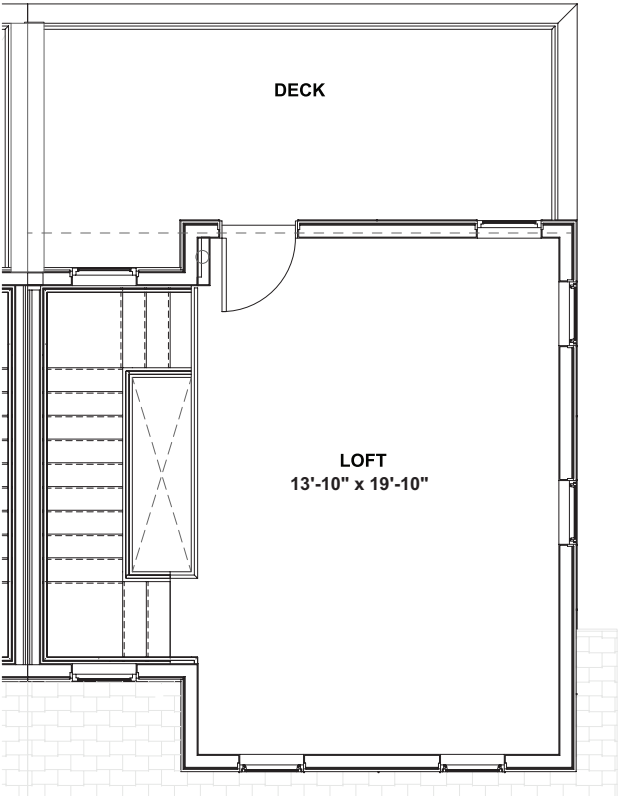
Third Floor
