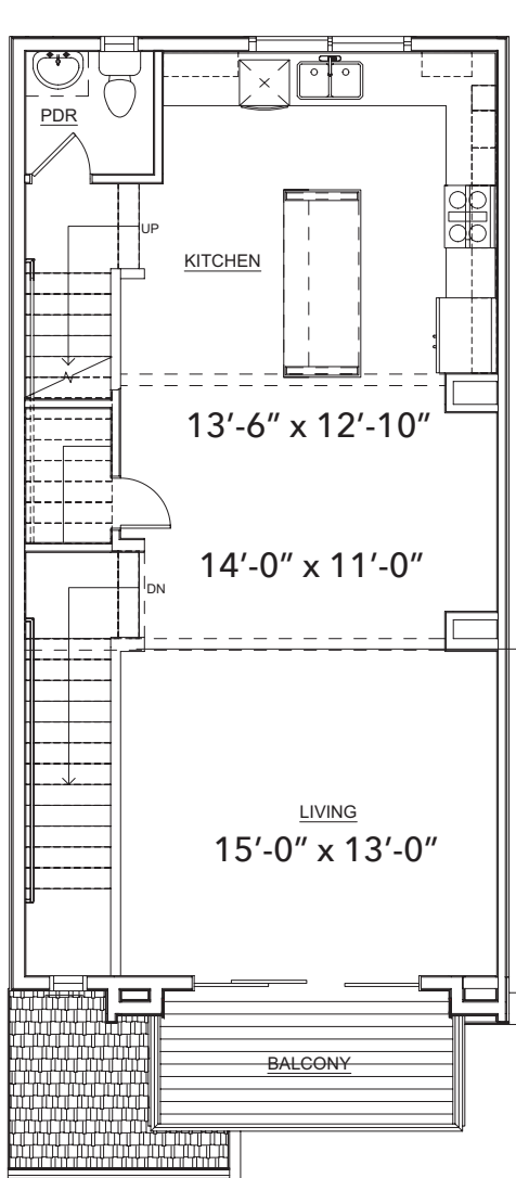
Second Floor Standard
