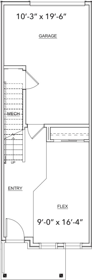
First Floor Flex
