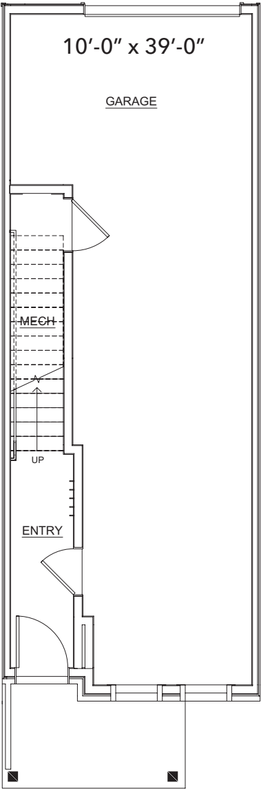
First Floor Standard
