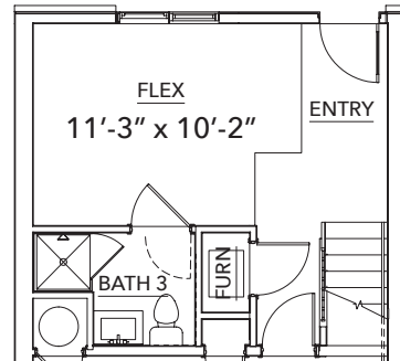
First Floor Bath Option
