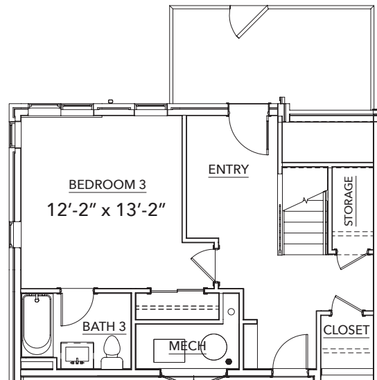
First Floor Bedroom/Bath Option
