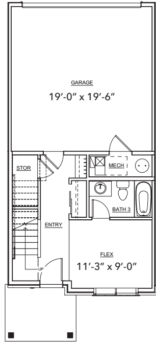
First Floor Bath & Flex
