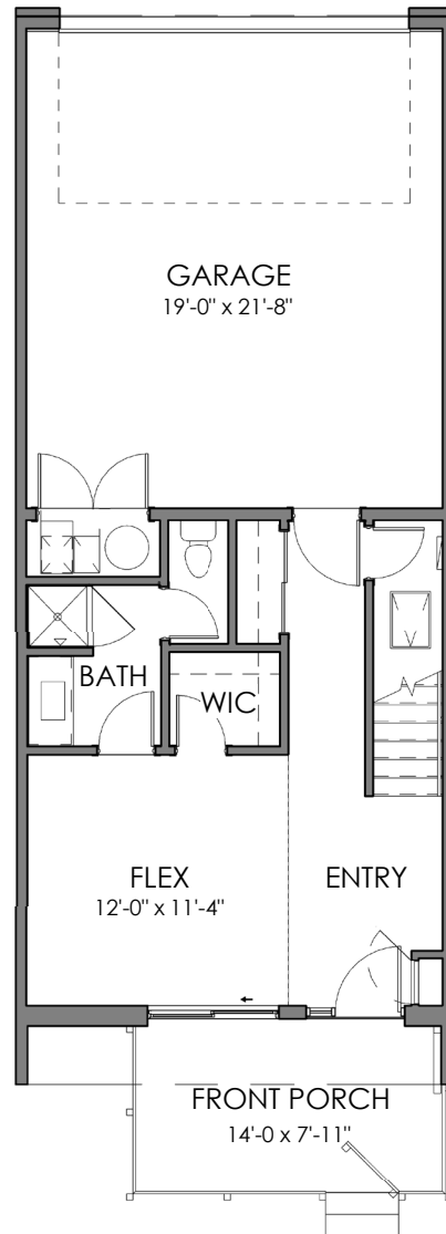
First Level with Optional Bath 446 Square Feet
