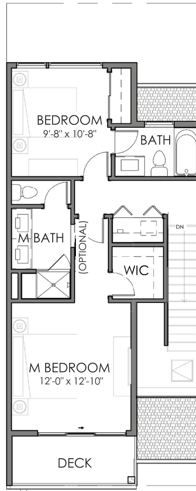
Third Level 615 Square Feet
