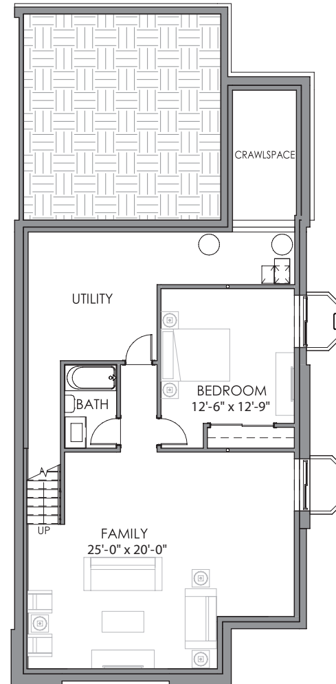
Optional Finished Basement 881 Finished Square Feet
