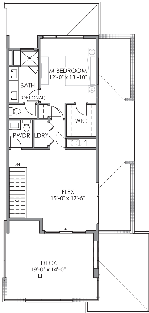
Second Level 779 Square Feet
