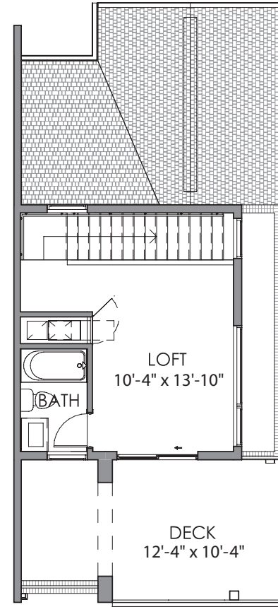
Third Level: 95 N. Pontiac Street 263 Square Feet
