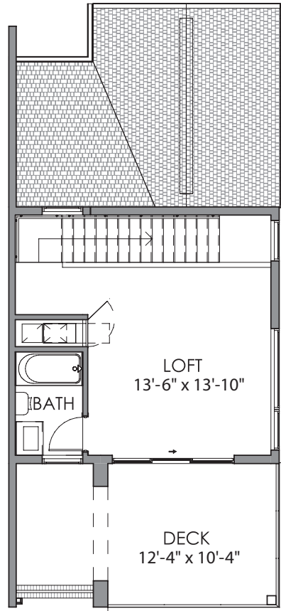
Third Level 316 Square Feet
